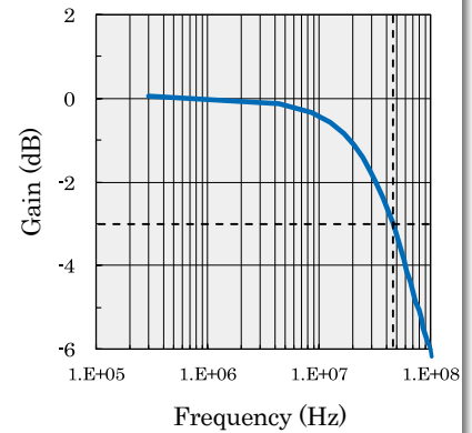
Fig6. Frequency Response
